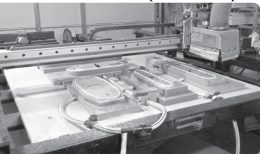
The CNC machine at cribbageboard.com.
